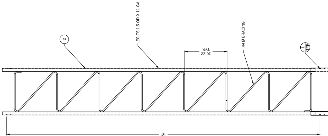
ELEVATION VIEW
